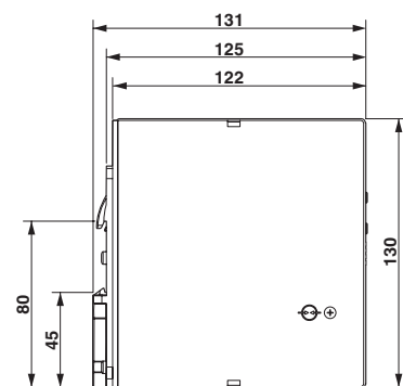
Dimensional drawing
